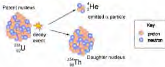
Alpha Decay of a Uranium-238 nucleus
